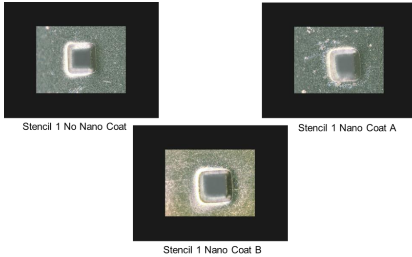
Figure 13 – Stencil 1 125 u Square Apertures 700x (Ranking Excellent – Points 4)
