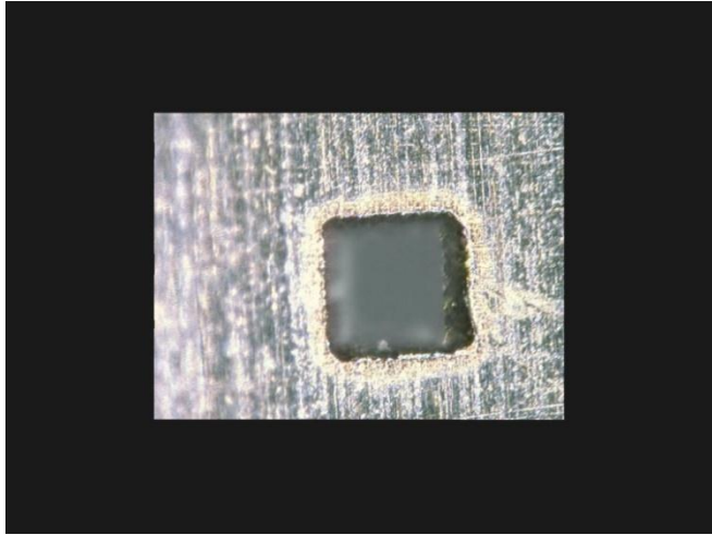
Stencil 4 No Nano Coat
