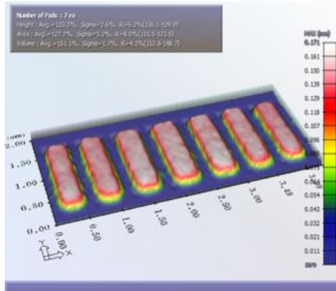
Good 2 Stencil 1 10th print (Nano-Coat B) 150 u Aperture
