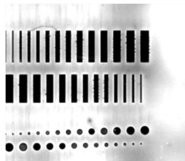
Figure 23 - Best Stencil for Bottom Side Paste Smear
