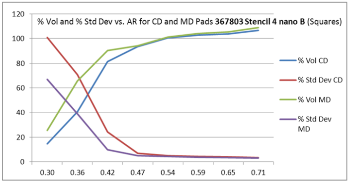
Figure 6 - 4 Stencils with Nano Coat B (Squares CD and MD)
