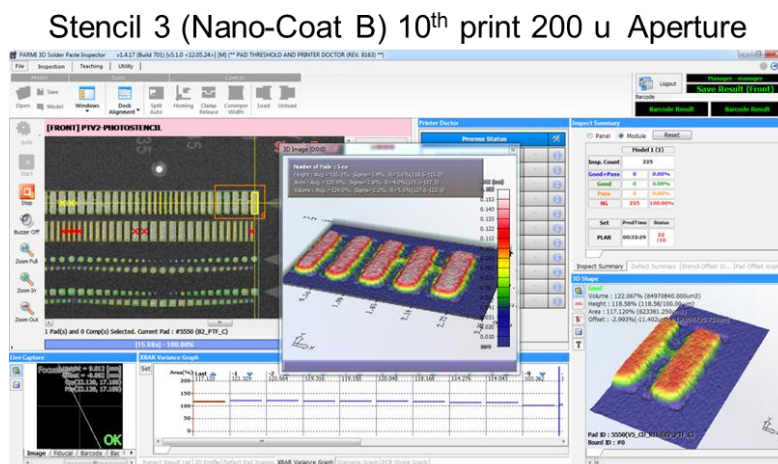
Figure 15 - Worst Performing Stencil
