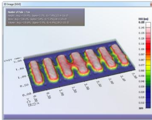
Good 2 Stencil 1 10th print (Nano-Coat B) 150 u Aperture
