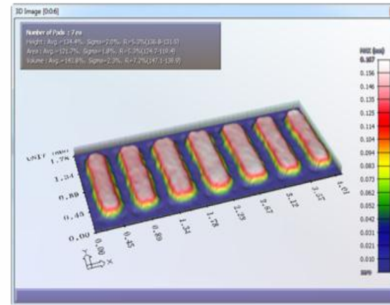
Good 2 Stencil 1 10th print no Nano-Coat 150 u Aperture
