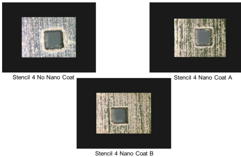
Figure 14 – Stencil 4 125 u Square Apertures 700x (Ranking Fair – Points 1)
