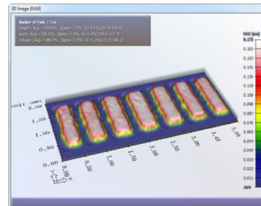
Good 2 Stencil 4 10th print (Nano-Coat A) 150 u Aperture
