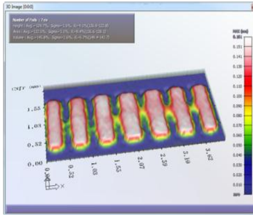
Good 2 Stencil 4 10th print no Nano-Coat 150 u Aperture
