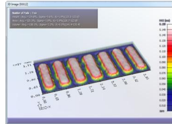
Good 2 Stencil 4 10th print (Nano-Coat A) 150 u Aperture
