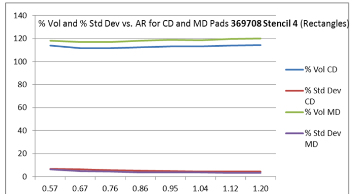
Figure 7 - 4 Stencils w/o Nano Coat (Rectangles CD and MD)
