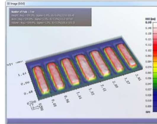
Poor 0 Stencil 4 10th print (Nano-Coat B) 150 u Aperture
