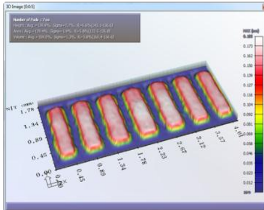
Good 2 Stencil 1 10th print (Nano-Coat A) 150 u Aperture
