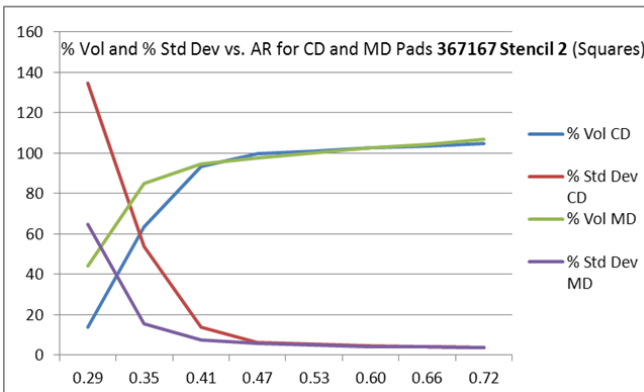
Figure 4 - 4 Stencils w/o Nano Coat (Squares CD and MD)
