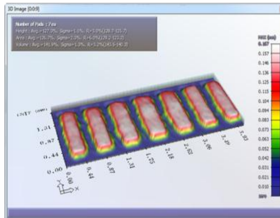
Good 2 Stencil 4 10th print no Nano-Coat 150 u Aperture
