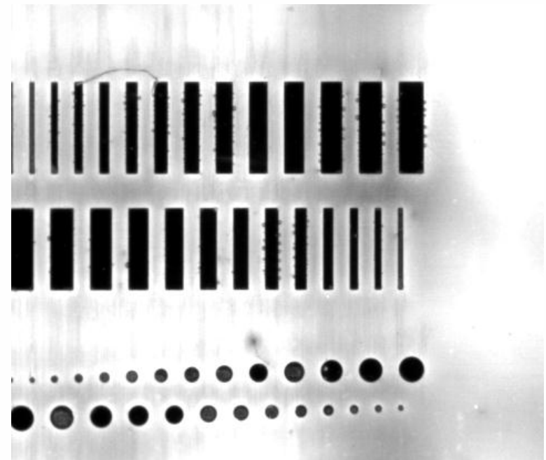
Stencil 2 10th print (Nano-Coat B)
